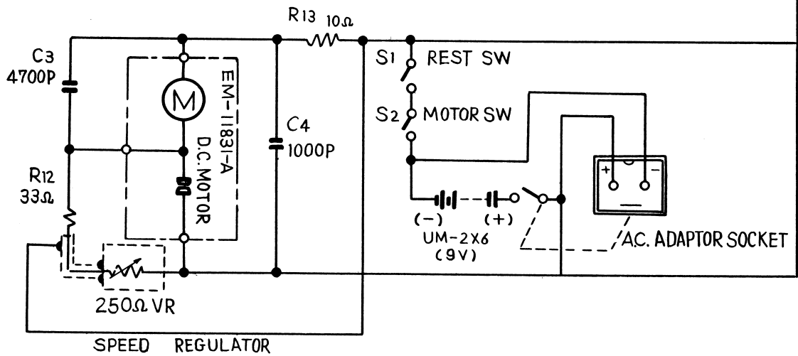
Schematic Diagram Model TPE-20
