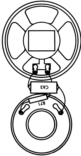
SPEAKER ASSEMBLY
