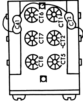
TRIMMER ASSEMBLY
