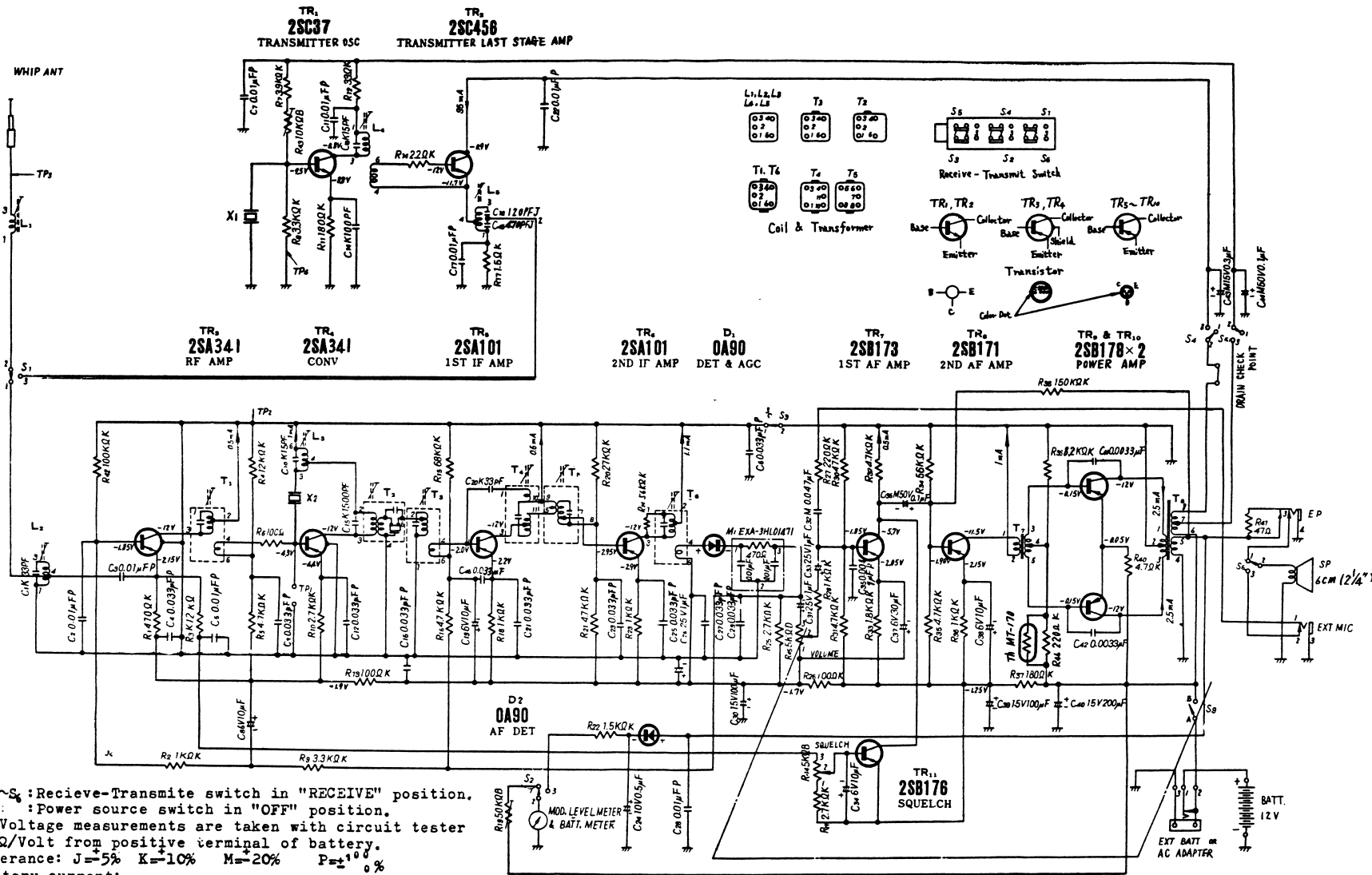
Fig. 1 Schematic Diagram.
