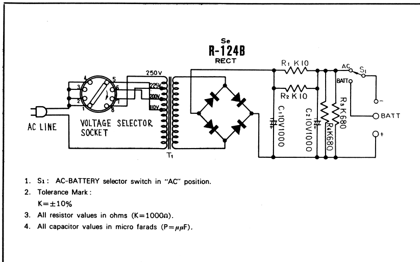
Fig. 18 Schematic Diagram.
