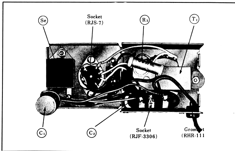
Fig. 19 Component View - Parts Identification.
