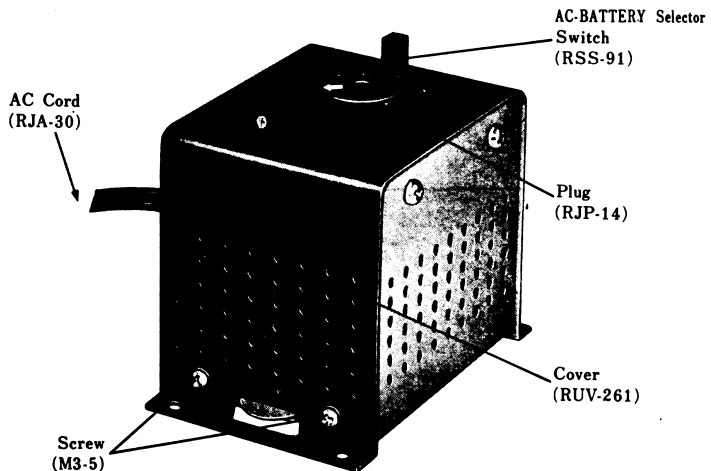
Fig. 17 Appearance - Parts Identification.
