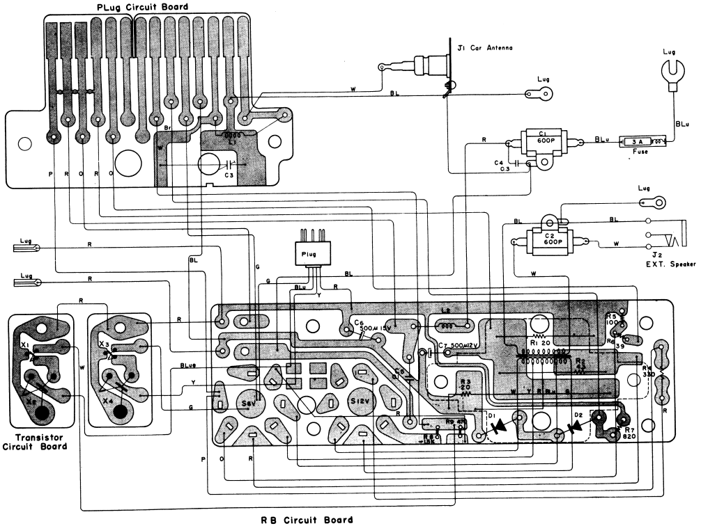
Mounting Diagram
