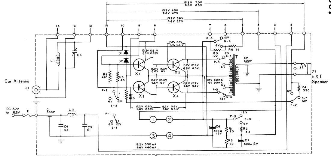
Change Polarity Diagram
