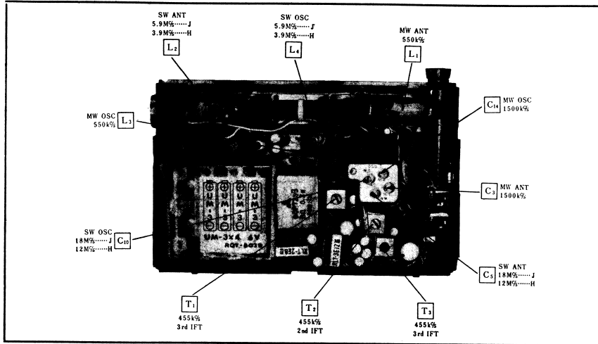
Fig. 5 Component View - Alignment Points.
