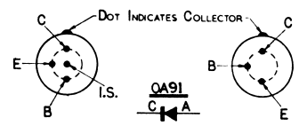
BOTTOM VIEW OF TRANSISTORS
