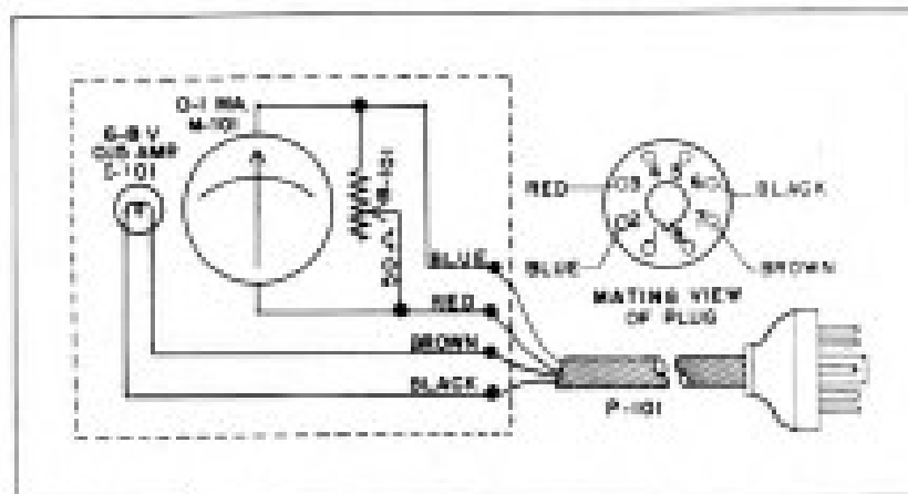
Figure No. 7. Schematic Diagram--SM-57 Tuning Meter
