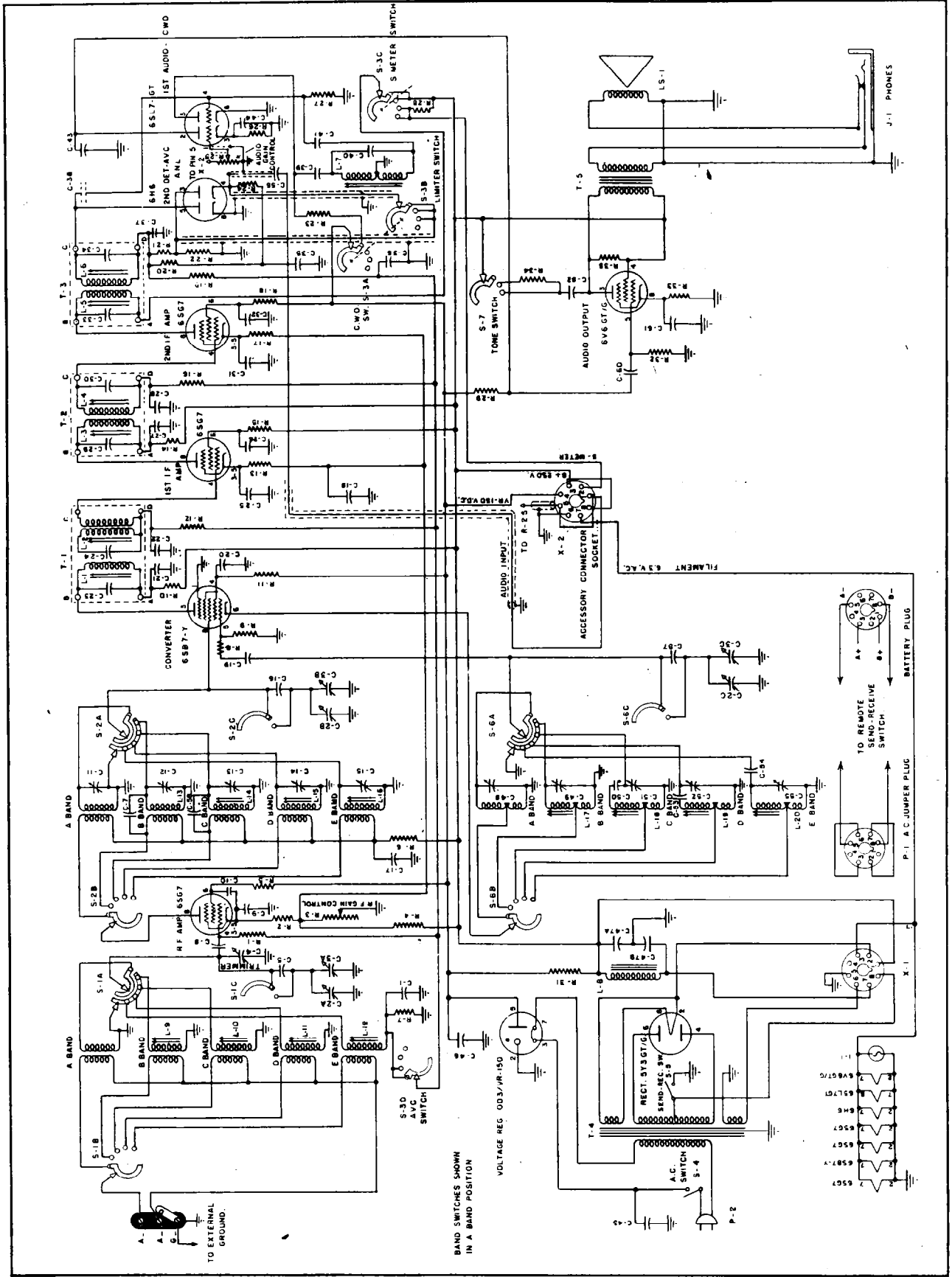
Figure No. 8. Schematic Diagram--NC-57 Receiver
