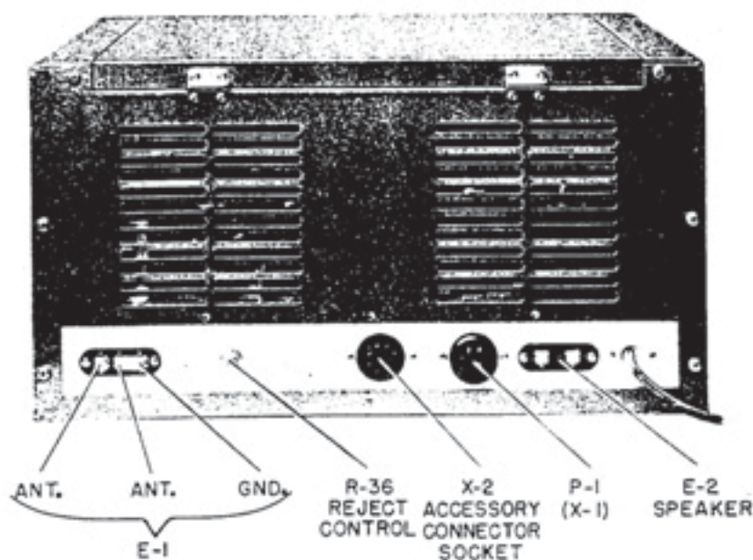
Figure No. 2. Rear View of Receiver
