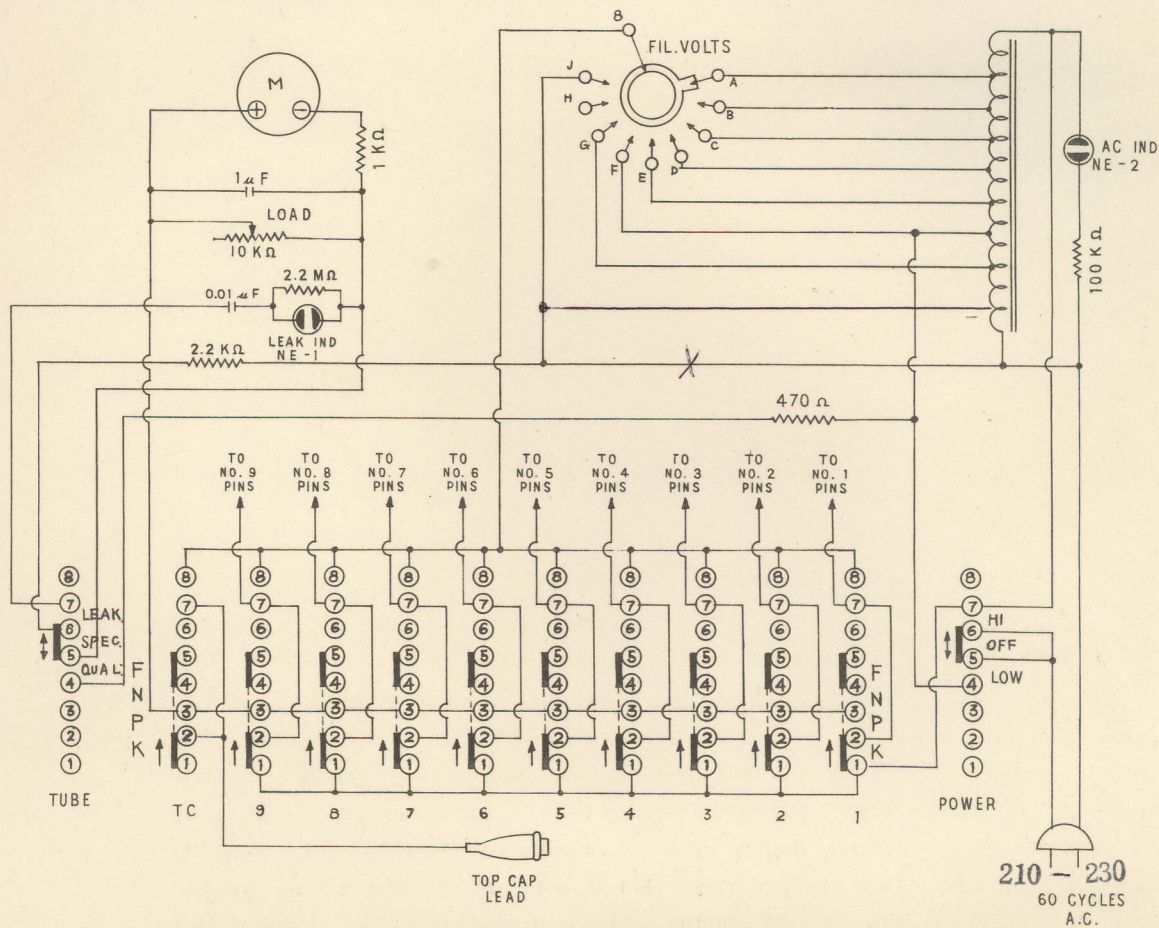
SCHEMATIC DIAGRAM
