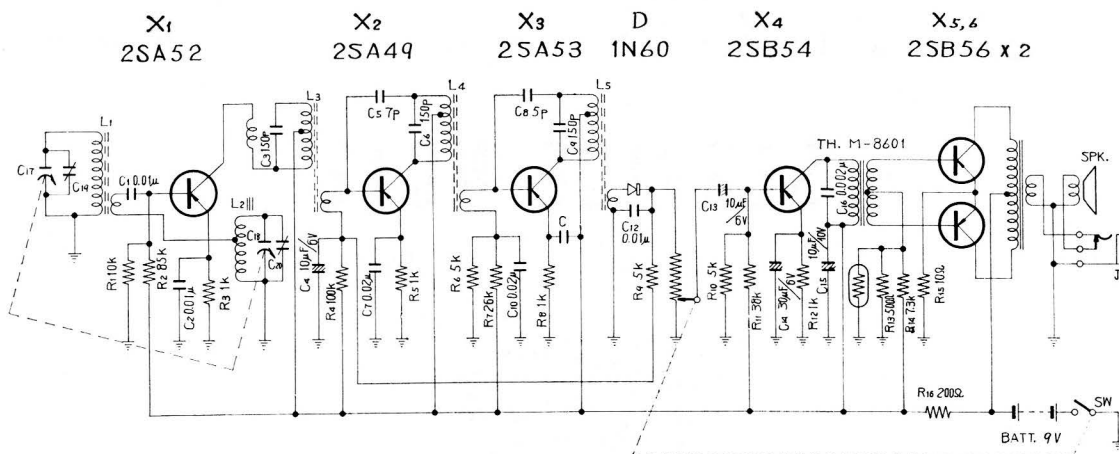
Schematic Diagram 6TB-4
