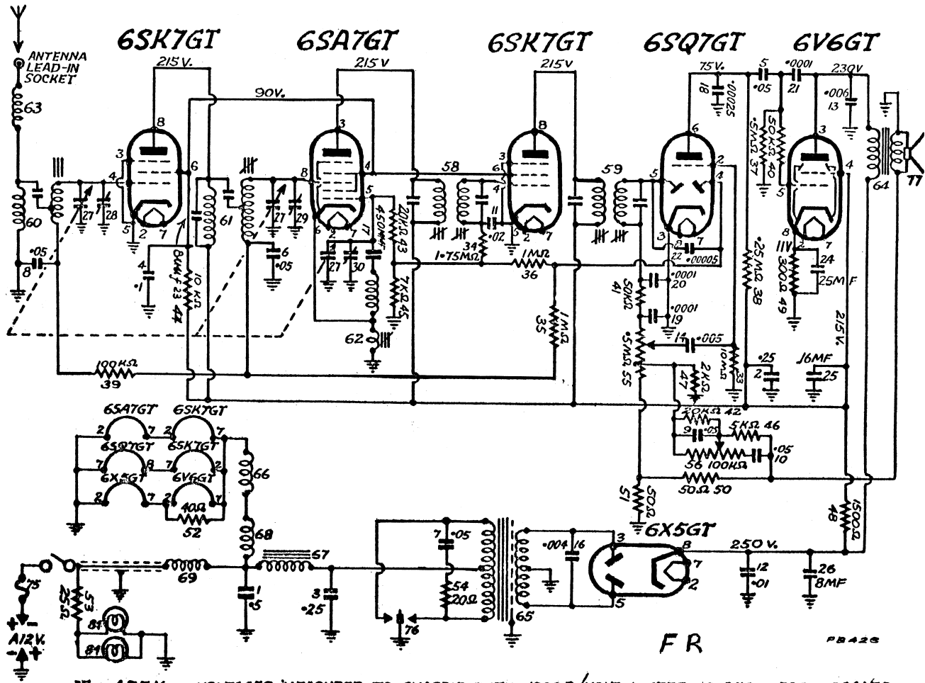
IF = 455 Kc.. VOLTAGES MEASURED TO CHASSIS WITH 1000 \Omega /VOLT METER 10, 250 & 500V. SCALES
