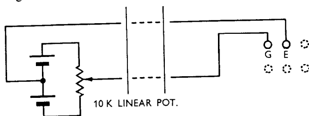
Fig. 5. Connections for Remote Oscillator Control.
