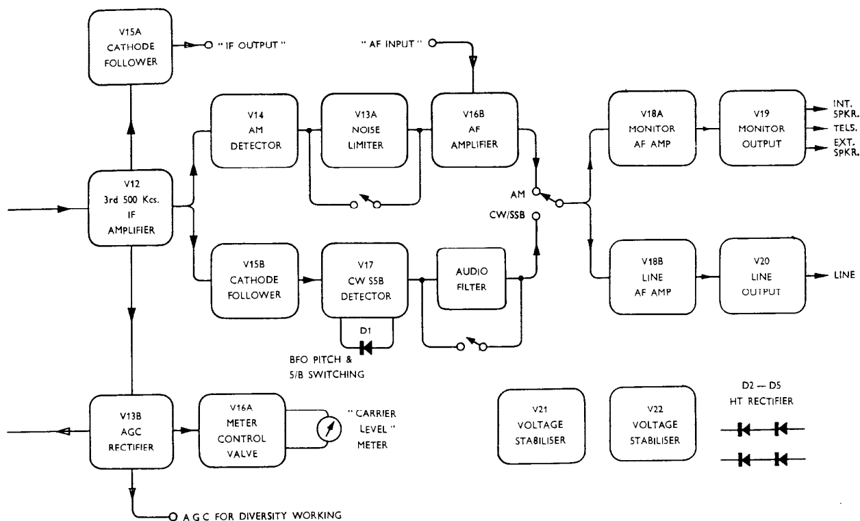
Fig. 3. Block Schematic Diagram — Model 880/2.
