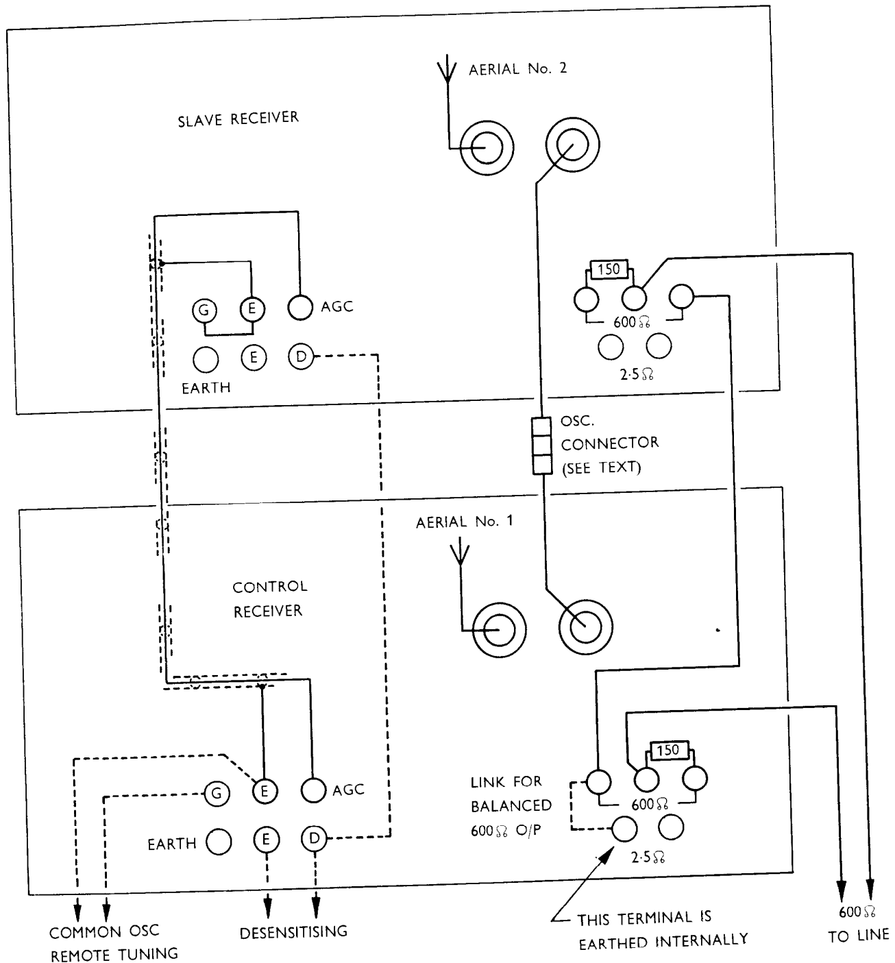
Fig. 6. Interconnection of two 880/2 receivers for dual diversity operation.
