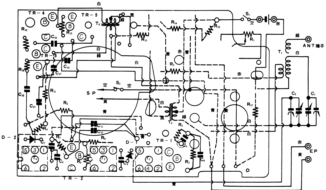
NATIONAL RADIO MODEL EB - 145
