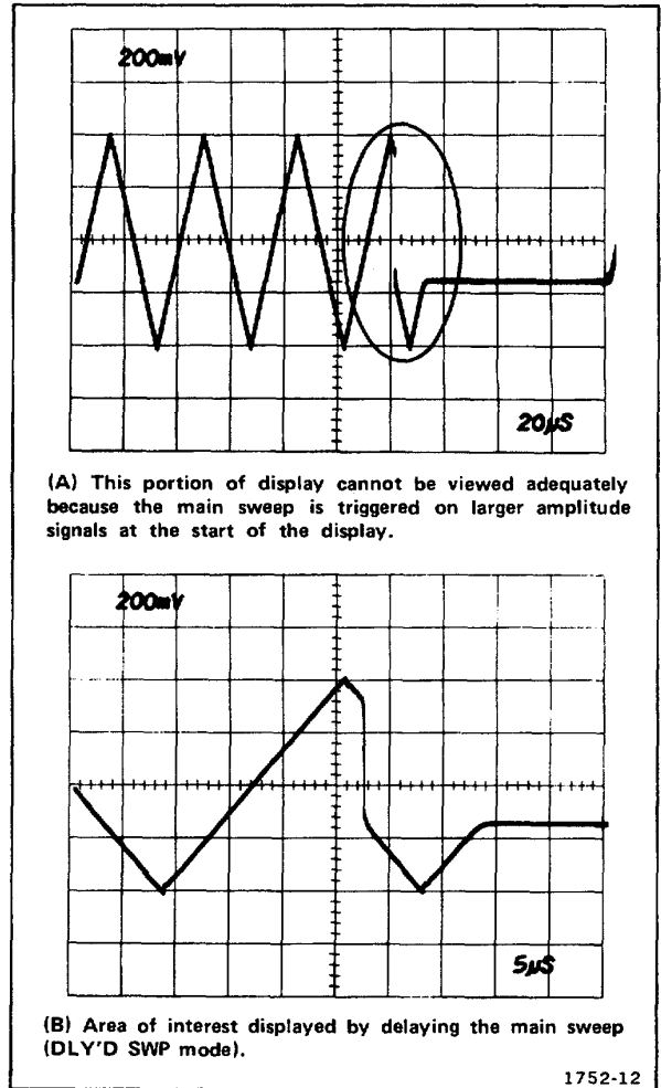
Figure 2-11. Displaying a complex signal using delayed sweep.
