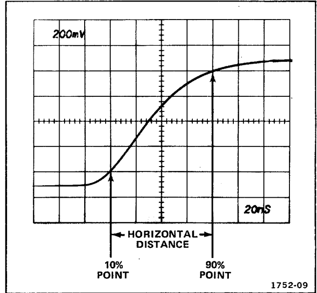
Figure 2-8. Measuring risetime.
