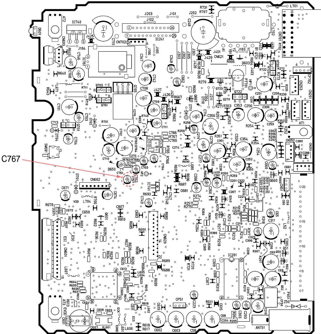
[E-6842Aa][Top View]
