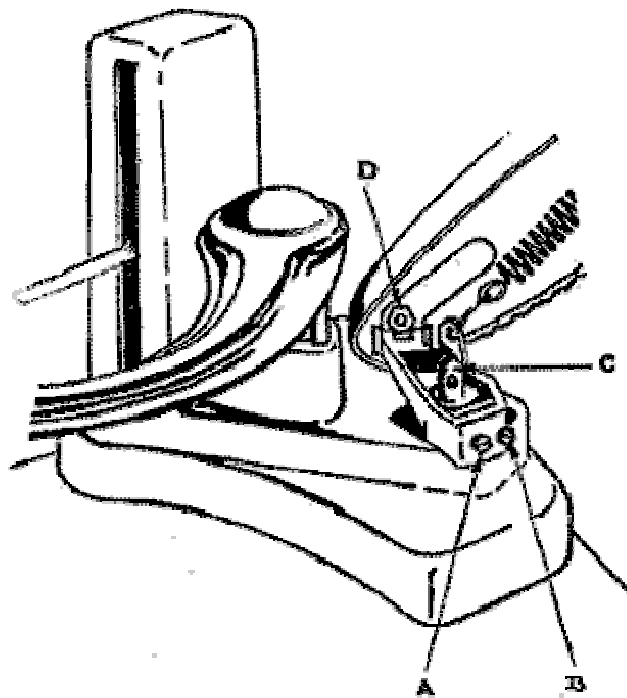
Fig. 2—View of Pick-up Housing with Pick-up Arm raised to reveal adjustments for Pick-up Position and height (Sections XII & XIII).
