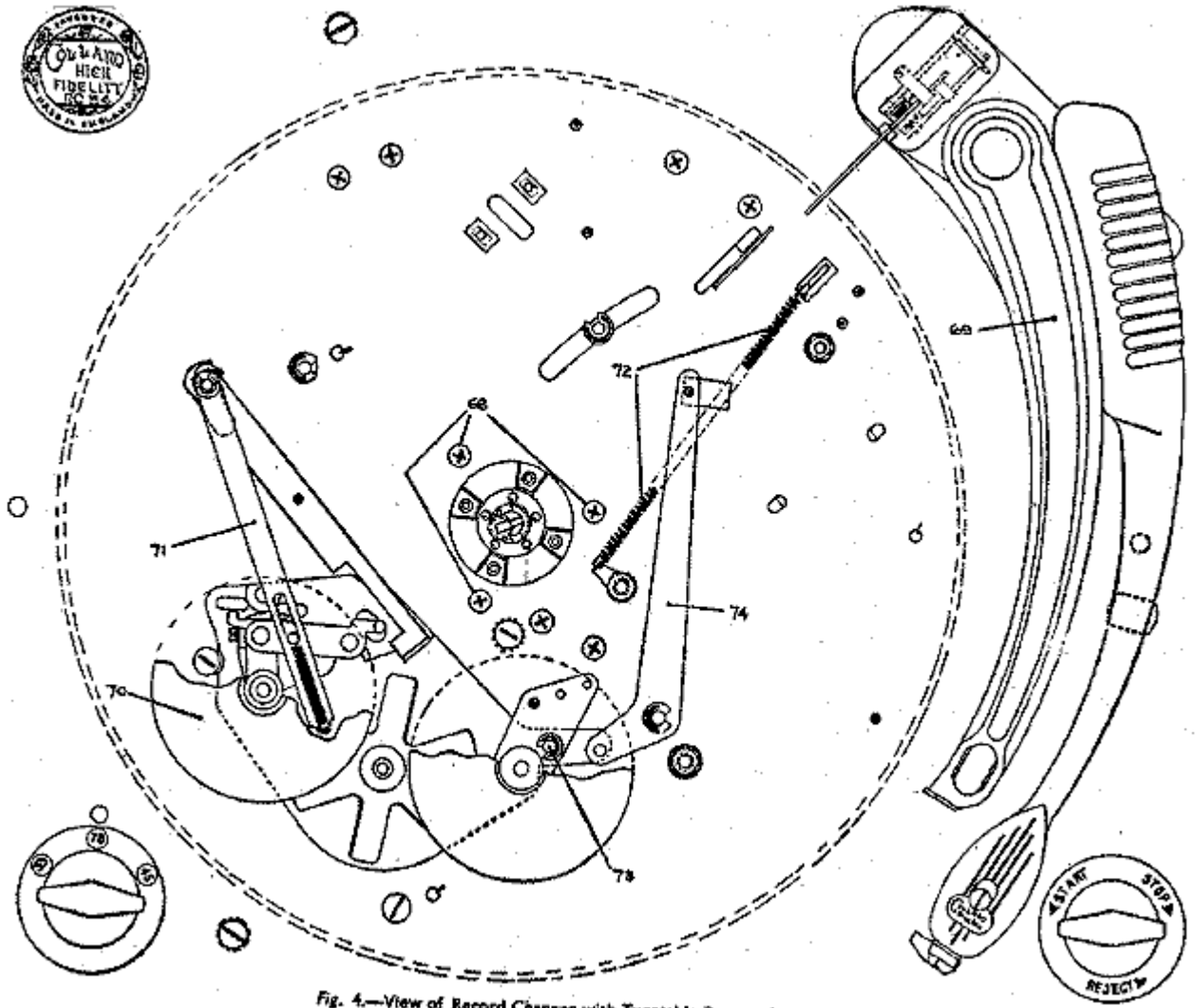
Fig. 4.—View of Record Changer with Turntable Removed
