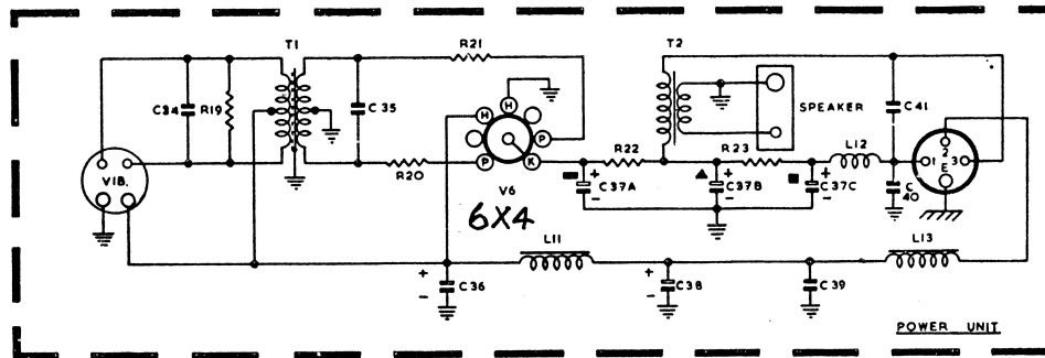
A.W.A. PRESSMATIC CAR RADIO (922, 923, 924, 925 SERIES EXCEPTING 924-B)
