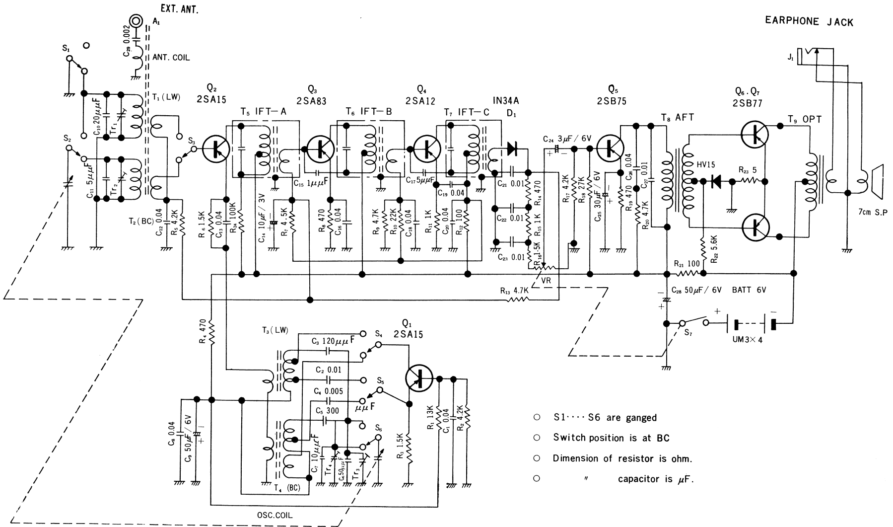
Mitsubishi MODEL 7X-970L CIRCUIT DIAGRAM
