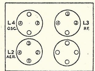
MANUAL TUNER REAR VIEW MODELS 2200/2400
