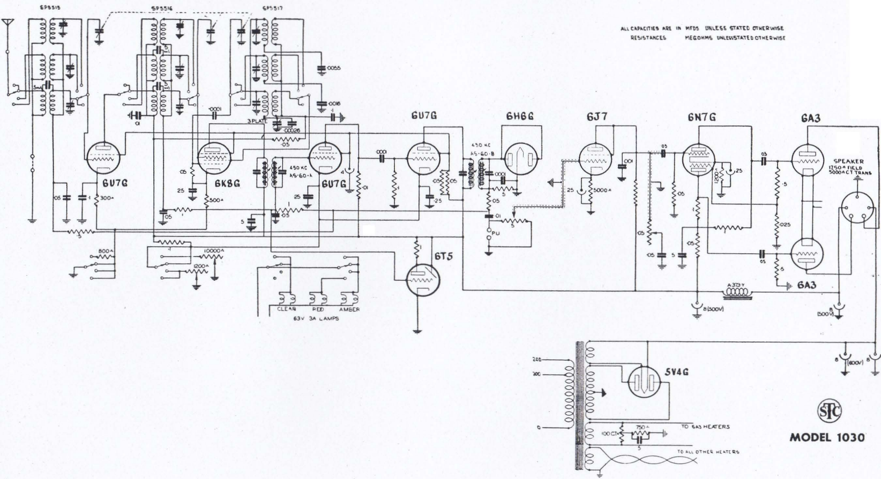
INTERMEDIATE FREQUENCY 450 K.C.
