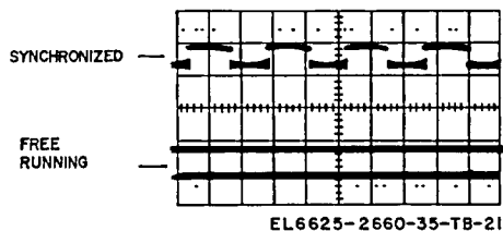
Figure 21. Trigger sensitivity.
