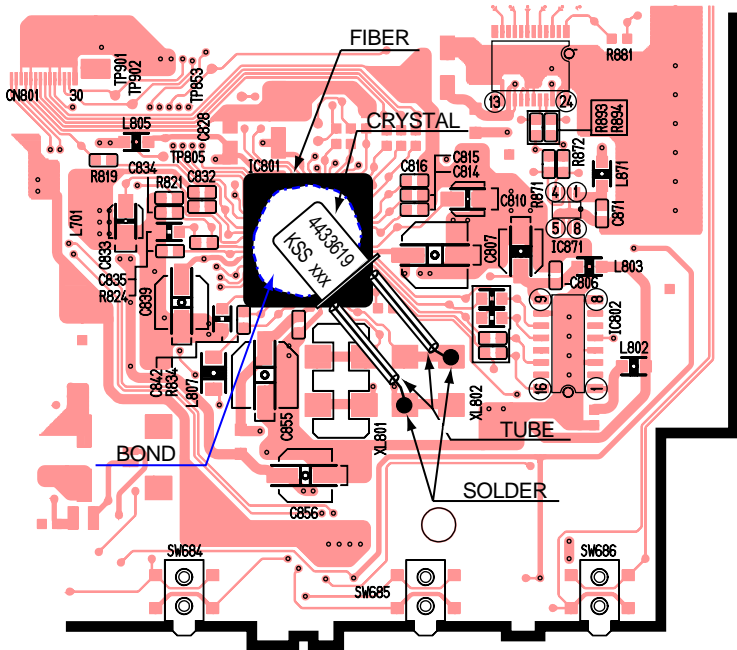
[E-8947B][Top View]
