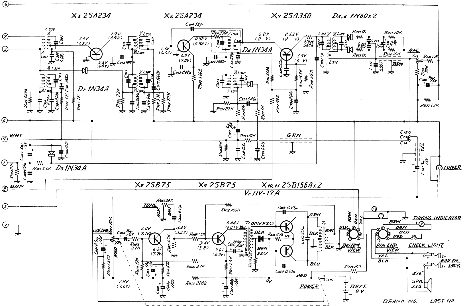
Schematic Diagram of IF & Audio Section
