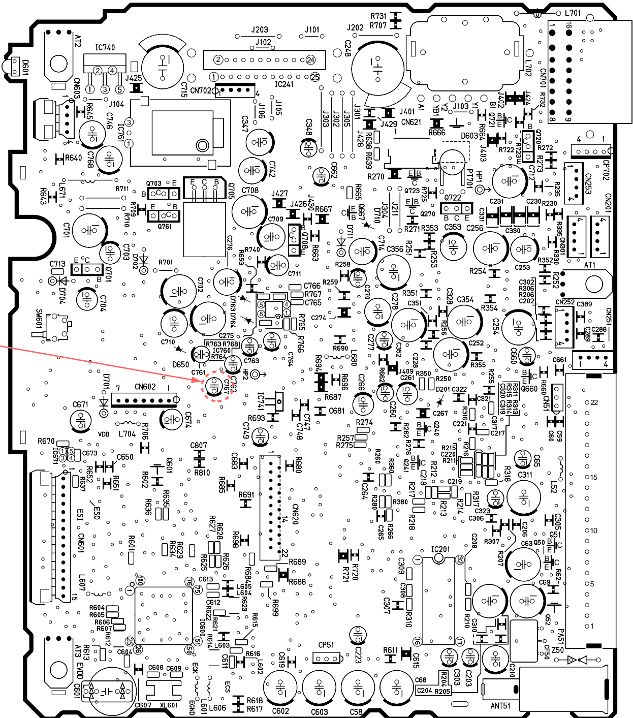
[E-6842Aa][Top View]
